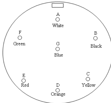
Solder Cup Side
